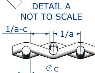
Plain Square Weave
