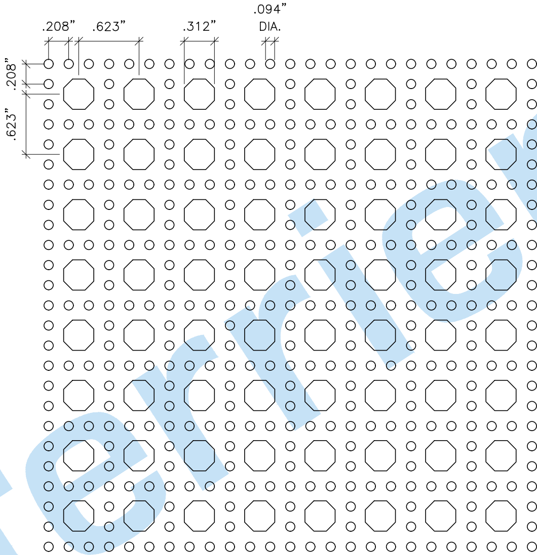
PLAN SCALE: FULL SIZE
